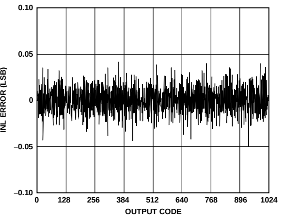
Figure 41. AD9600 INL with f_{IN1} = 10.3 MHz
