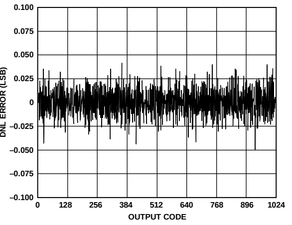
Figure 42. AD9600 DNL with f_{IN1} = 10.3 MHz
