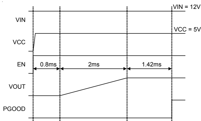
Figure 1. Soft-Start Sequence
