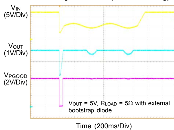
Starting Profile III (Cold cranking)
