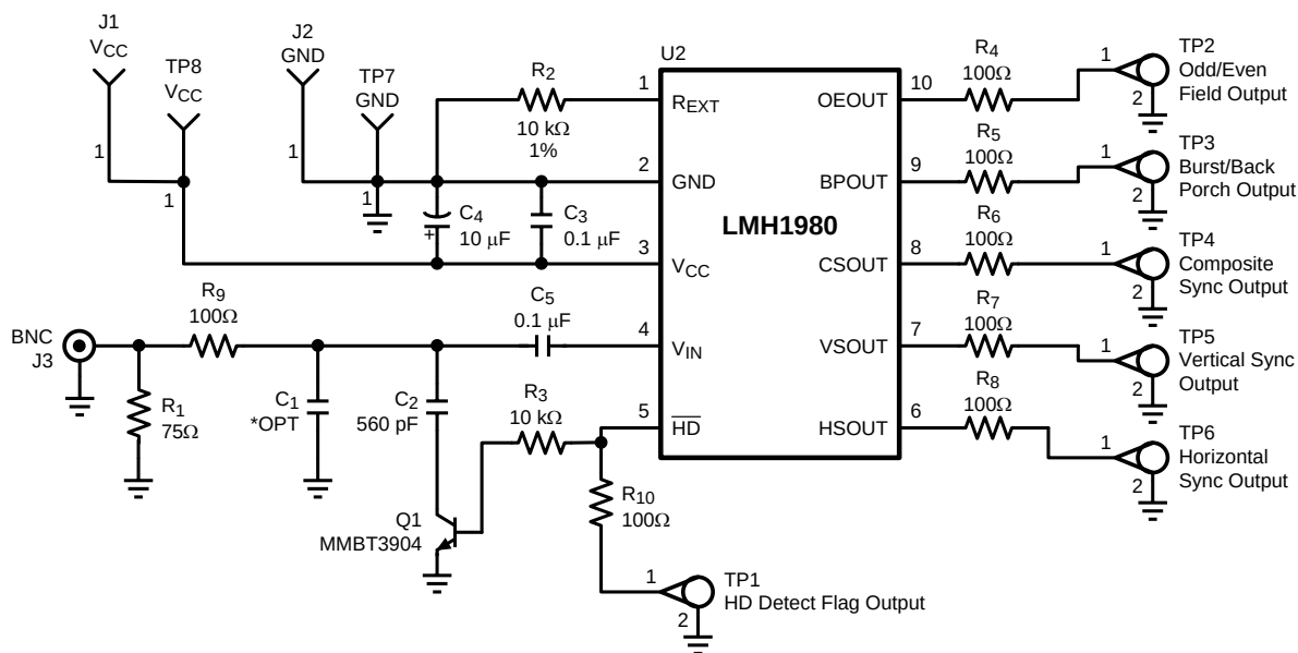
Figure 2. Test Circuit
