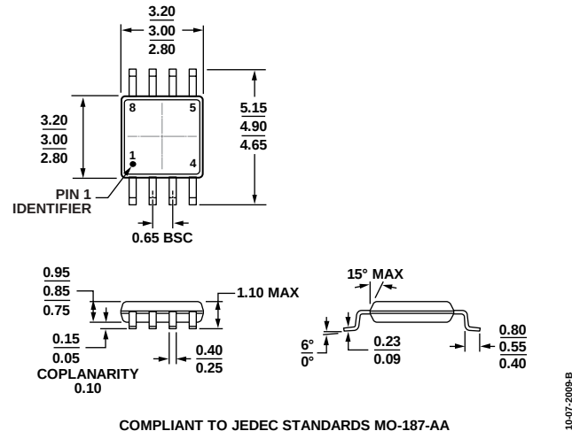
Figure 75. 8-Lead Mini Small Outline Package [MSOP] (RM-8) Dimensions shown in millimeters
