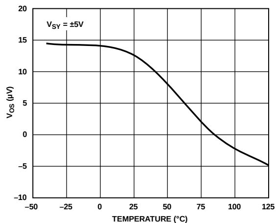
Figure 13. Offset Voltage ( V_{OS} ) vs. Temperature, V_{SY} = \pm 5V
