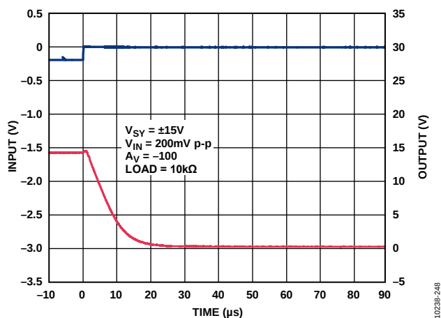
Figure 51. Positive Overload Recovery, V_{SY} = \pm 15\text{ V}
