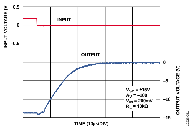
Figure 52. Negative Overload Recovery, V_{SY} = \pm 15\text{ V}
