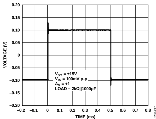
Figure 50. Small Signal Transient Response, V_{SY} = \pm 15\text{ V}
