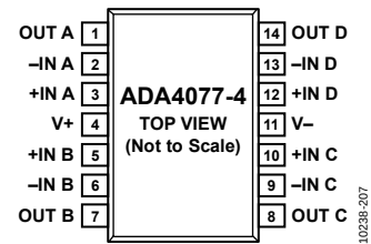
Figure 10. ADA4077-4 Pin Configuration, 14-Lead SOIC
