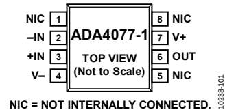
Figure 1. ADA4077-1, 8-Lead SOIC and 8-Lead MSOP
