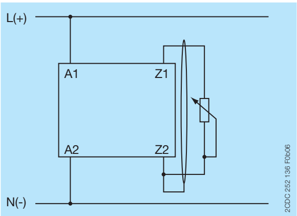
Remote potentiometer
