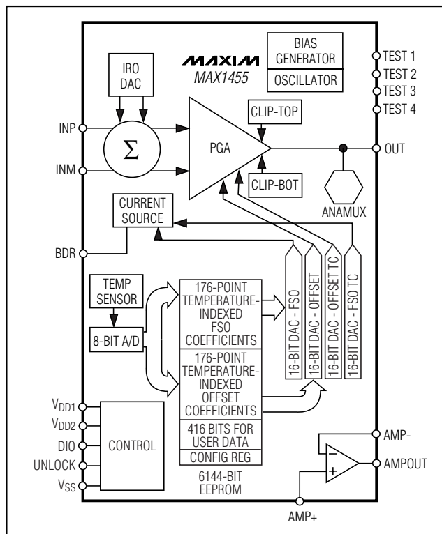
Figure 1. Functional Diagram
