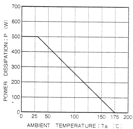
Fig. 4 Derating curve
