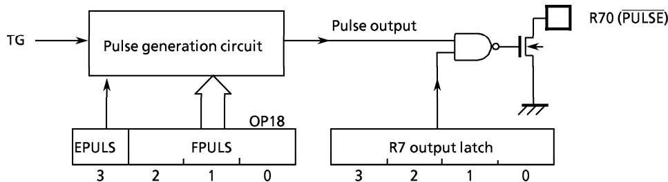
Figure 3-4. Pulse output circuit
