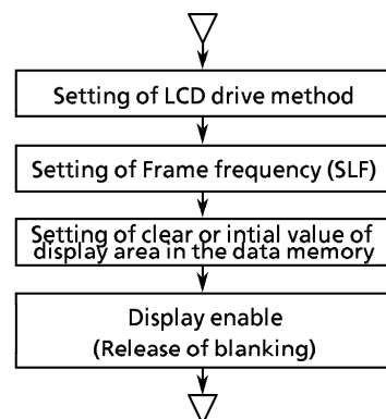
Figure 3-10. Intial setting of LCD driver
