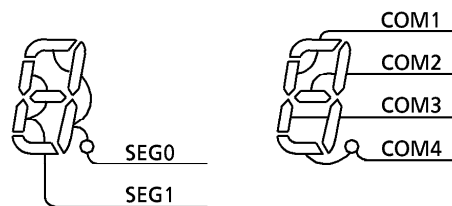
Figure 3.11 Example of COM. and SEG connection
