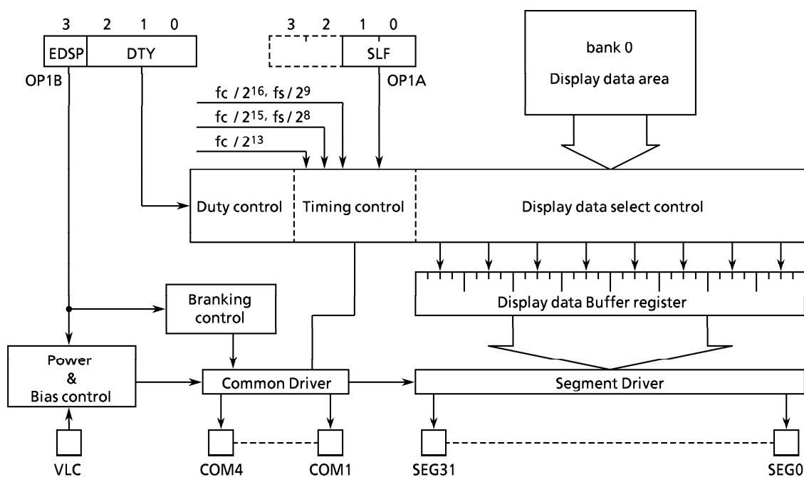
Figure 3-6. LCD Driver
