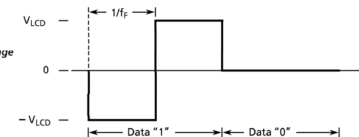
Figure 3-8. LCD drive waveform (COM-SEG pins)
