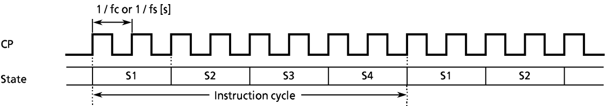
Figure 2-3. Instruction Cycle
