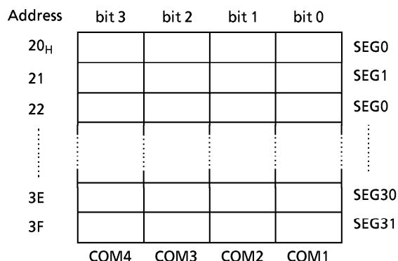
Figure 3-9. LCD Display Data Area (Bank 0)
