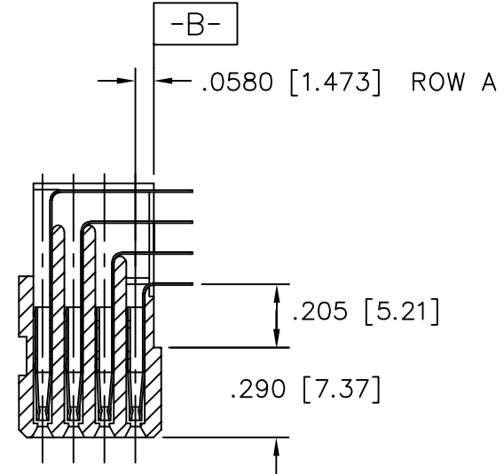
SECTION X-X
