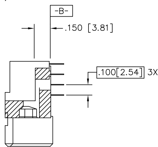
SECTION U-U
