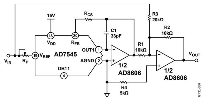
Figure 56. Bipolar Operation
