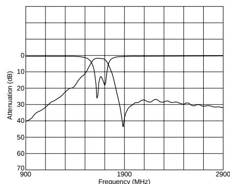
Frequency Characteristics
