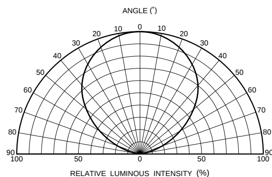
Fig.1 Directional pattern
