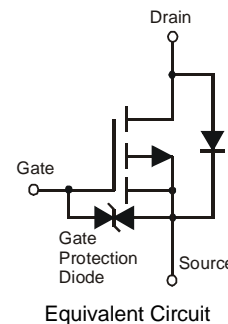
Equivalent Circuit
