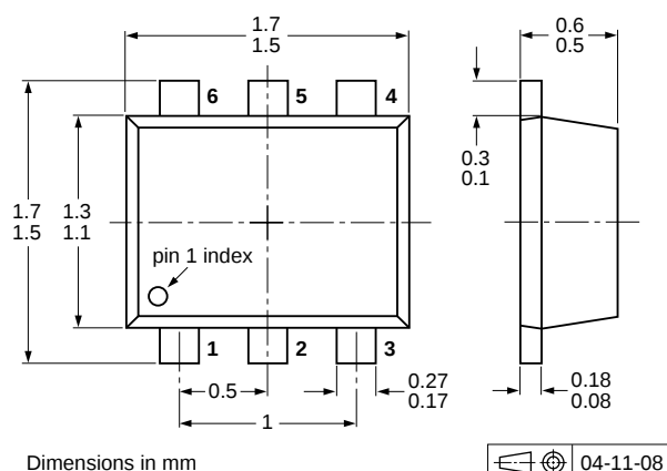
Fig 10. Package outline PEMB18 (SOT666)
