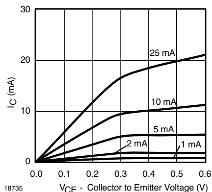
Figure 5. Normalized Current vs. Collector Emitter Saturation Voltage
