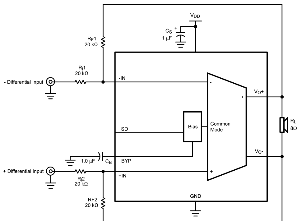
Figure 10. Audio Block
