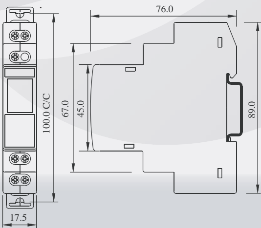
MOUNTING DIMENSIONS (mm)
