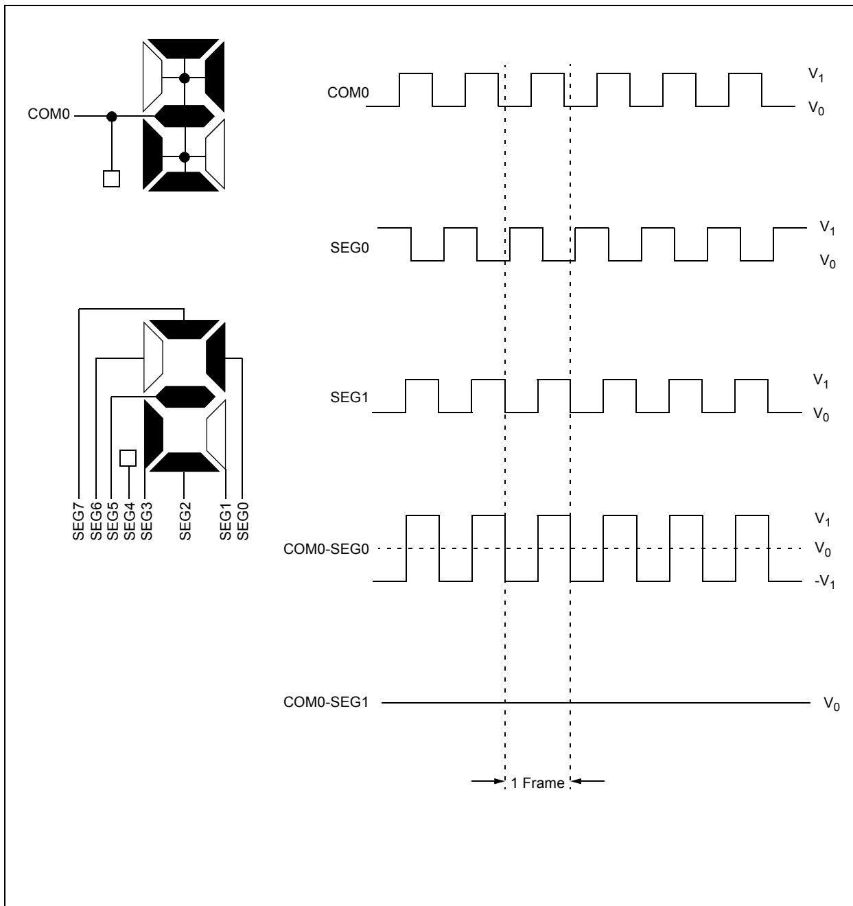
FIGURE 22-4: TYPE-A/TYPE-B WAVEFORMS IN STATIC DRIVE
