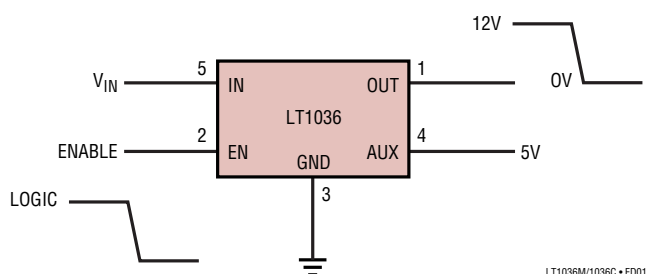
Functional Diagram
