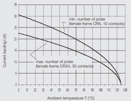
ConCept module CM-5 Conductor H07V-K 4.0 mm²
