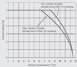
ConCept module CM-5 Conductor H05V-K 0.5 mm²
