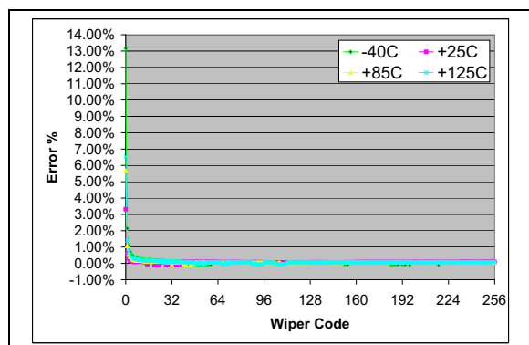
FIGURE 2-59: 100 kΩ – Worst Case R_{BW} from Average R_{BW} ( R_{BW0} - R_{BW3} ) Error (%) vs. Wiper Setting and Temperature ( V_{DD} = 5.5\text{V} , I_W = 45\text{ }\mu\text{A} ).
