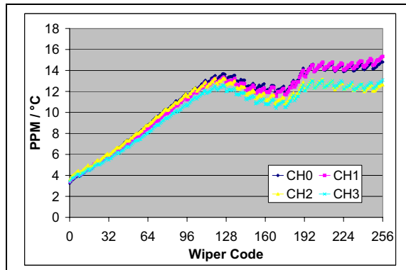
FIGURE 2-62: 100 kΩ – R_{WB} PPM/ ^\circ\text{C} vs. Wiper Setting. ( R_{BW(\text{code}=n, 125^\circ\text{C})} - R_{BW(\text{code}=n, -40^\circ\text{C})} / R_{BW(\text{code}=256, 25^\circ\text{C})} / 165^\circ\text{C} * 1,000,000 ) ( V_{DD} = 3.0\text{V} , I_W = 24\text{ }\mu\text{A} ).
