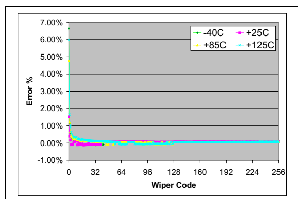
FIGURE 2-60: 100 kΩ – Worst Case R_{BW} from Average R_{BW} ( R_{BW0} - R_{BW3} ) Error (%) vs. Wiper Setting and Temperature ( V_{DD} = 3.0\text{V} , I_W = 24\text{ }\mu\text{A} ).
