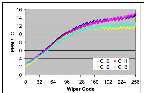
FIGURE 2-61: 100 kΩ – R_{WB} PPM/ ^\circ\text{C} vs. Wiper Setting. ( R_{BW(\text{code}=n, 125^\circ\text{C})} - R_{BW(\text{code}=n, -40^\circ\text{C})} / R_{BW(\text{code}=256, 25^\circ\text{C})} / 165^\circ\text{C} * 1,000,000 ) ( V_{DD} = 5.5\text{V} , I_W = 45\text{ }\mu\text{A} ).
