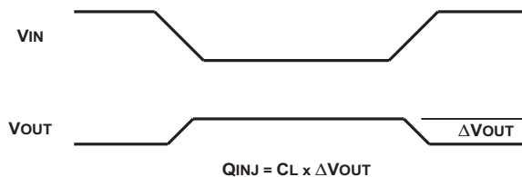
Figure 5. Charge Injection
