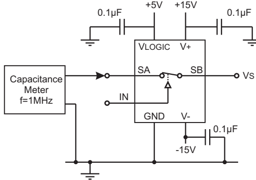
Figure 9 - On Capacitance
