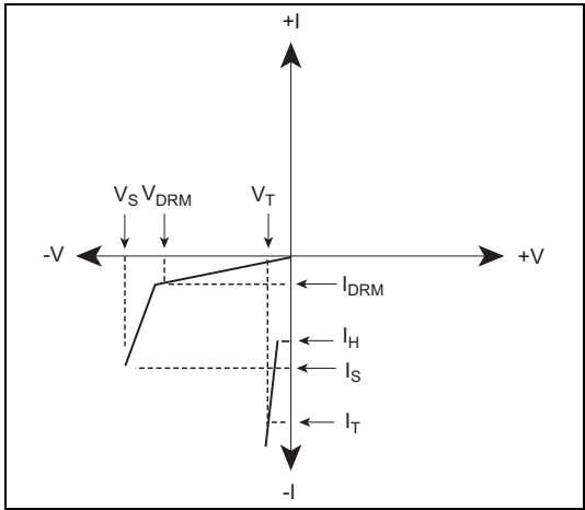
V-I Characteristics for Negative Battrax
