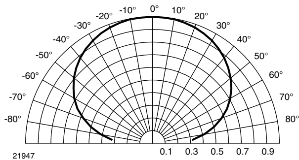
Fig. 11 - Horizontal Directivity
