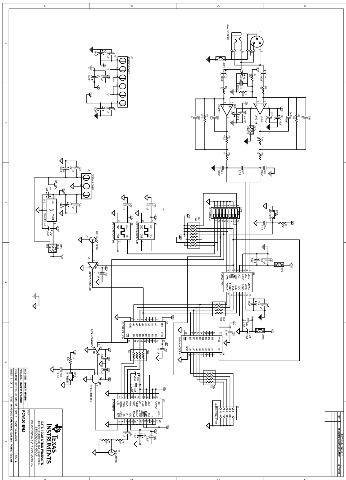
Figure 4. PCM4201EVM Schematic
