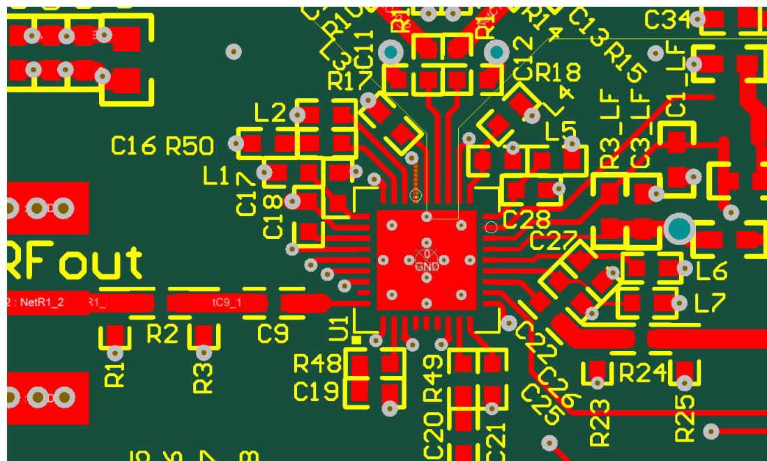
Figure 43. Layout
