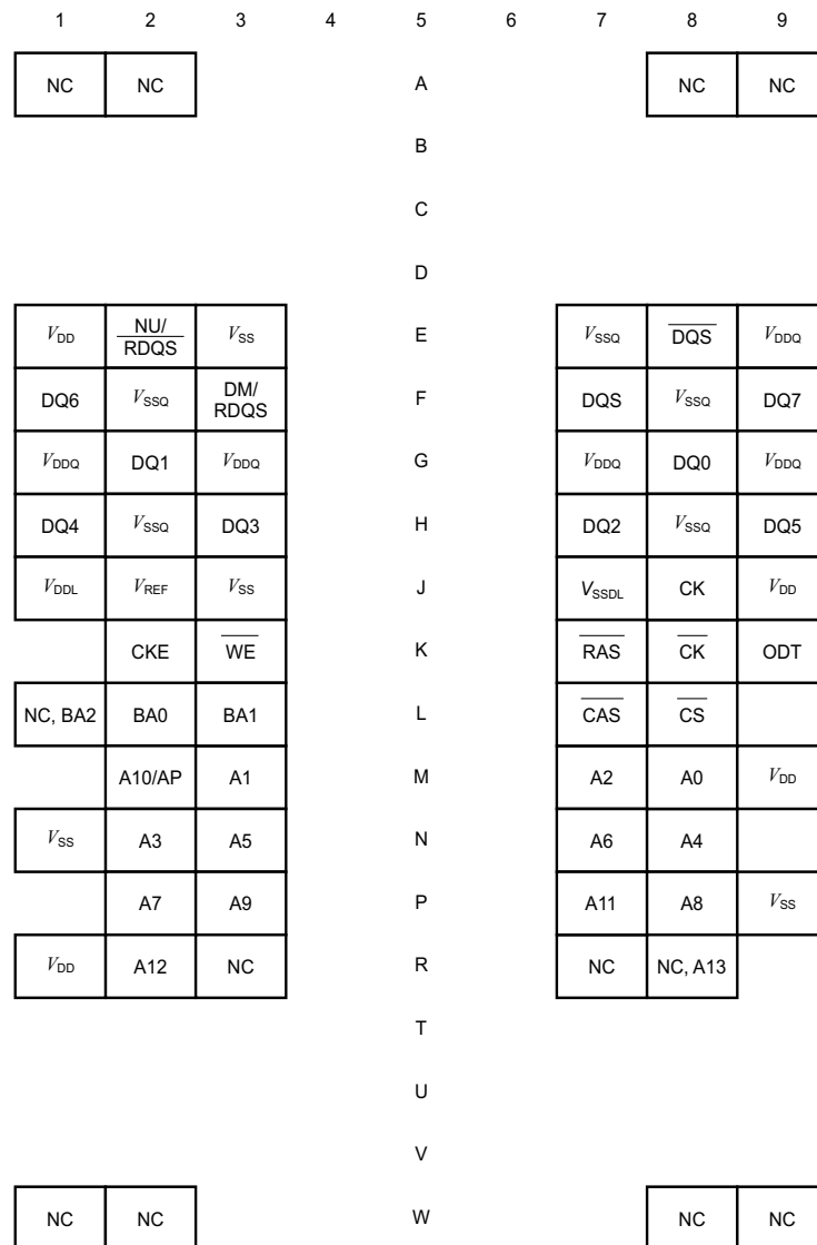
FIGURE 1 Ball Configuration for ×8 components, PG-TFBGA-68 (top view)
