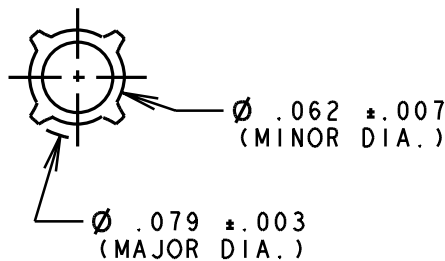
DETAIL "A" (2 PLCS) SCALE 8:1
