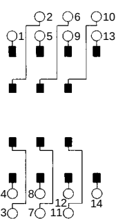
Schematic
