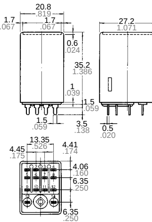
HC4-H (4 Form C)
