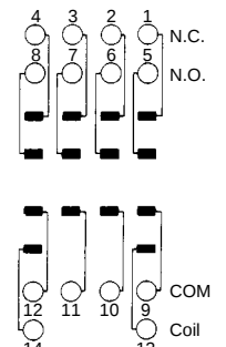
Schematic
