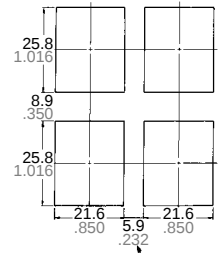
Chassis cutout
