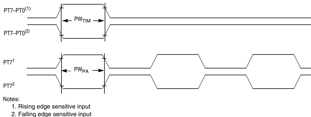
Figure 19-5. Timer Inputs
