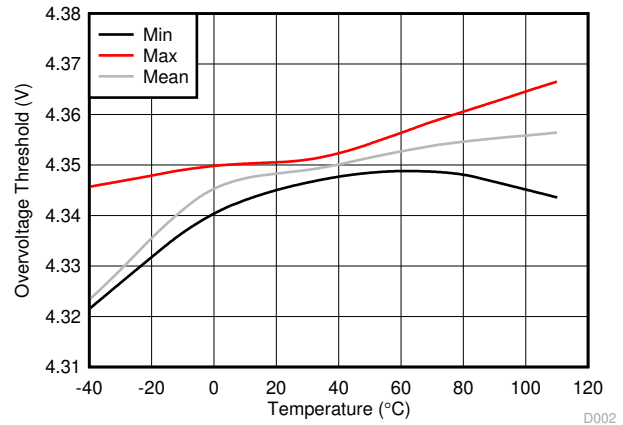
Figure 7-2. BQ294502 Overvoltage Threshold (OVT) vs Temperature
