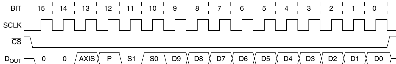
Figure 4-5 Acceleration Command Response
