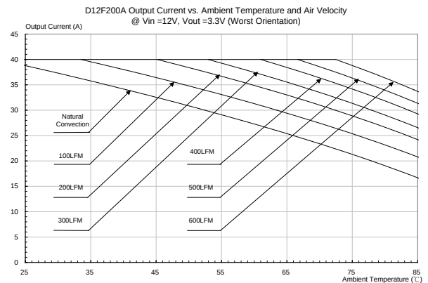
Figure 39: Output current vs. ambient temperature and air velocity @ Vin=12V, Vout=3.3V (Worst Orientation)
