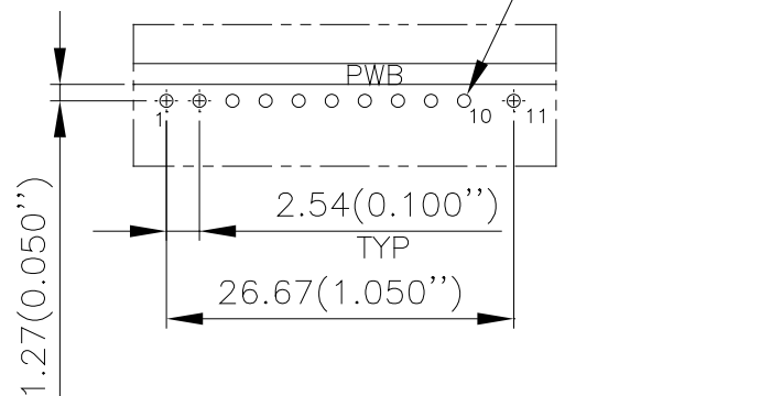
RECOMMENDED PWB LAYOUT
