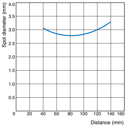
Spot Diameter vs. Sensing Distance Narrow-beam Reflective Models E3Z-L□1(L□6)
