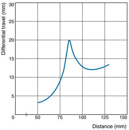
Differential Travel vs. Sensing Distance Narrow-beam Reflective Models E3Z-L□1(L□6)
