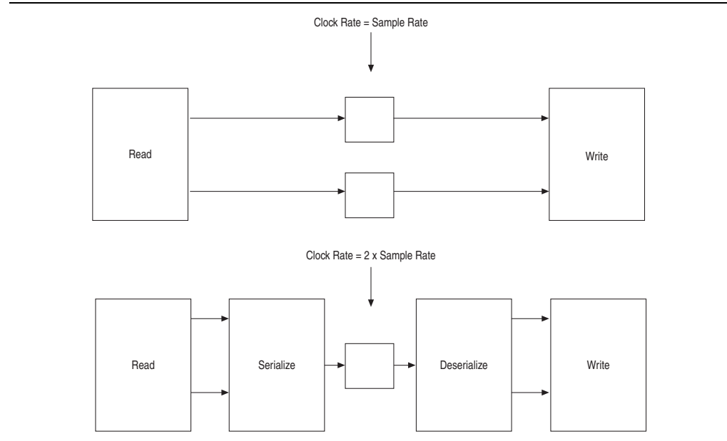
Figure 4-8. Time-Division Multiplexing to Save Hardware Resources
