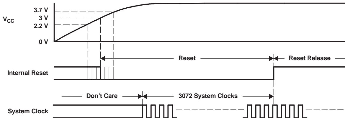
Figure 21. Power-On-Reset Timing
