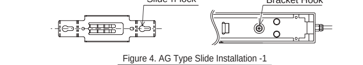
Figure 4. AG Type Slide Installation -1
