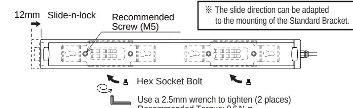
Figure 7. AG Type Slide Installation -2
