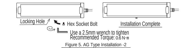
Figure 5. AG Type Installation -2
