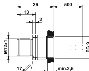
M12 flush-type plug, can be positioned
