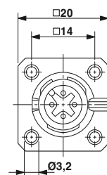
M12 flush-type plug, square flange
