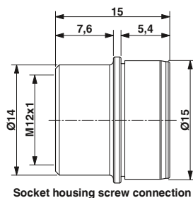
Socket housing screw connection
