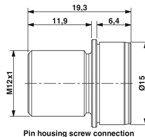
Pin housing screw connection
