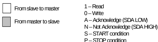
Figure 23. I 2 C Write Operation
