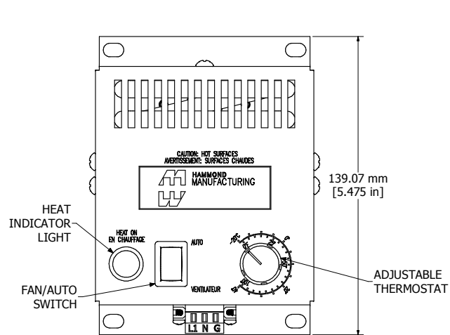
ASSEMBLY - VIEW FROM FRONT
