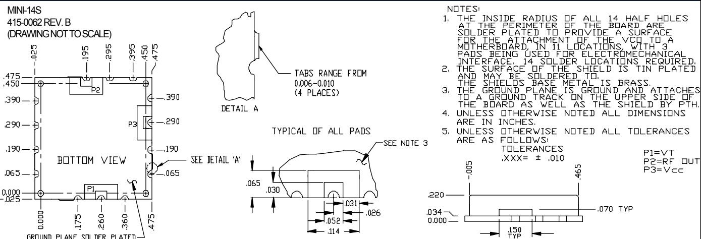
PHYSICAL DIMENSIONS
