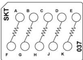
CTJ420E037 Five 23.2 kOhm Resistors, 1/20 W
