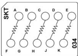
CTJ420E034 Five 150 Ohm Resistors, 1/10 W
