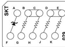
CTJ420E029 Two 10 kOhm Resistors, 1/10 W Two 1.43 kOhm Resistors, 1/10 W One JANTX 1N4954 Zener Diode
