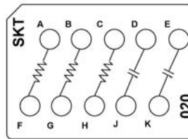
CTJ420E020 Two 3.6 kOhm Resistors, 1/10 W One 100 kOhm Resistor, 1/10 W Two 1 uF Capacitors, 50 WVDC
