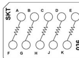
CTJ420E036 Five 2.8 kOhm Resistors, 1/10 W
