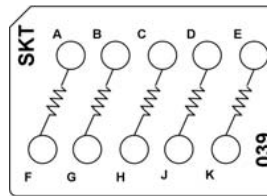
CTJ420E039 Five 41.2 kOhm Resistors, 1/20 W
