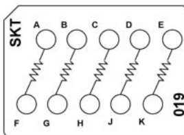
CTJ420E019 One 1.10 kOhm Resistor, 1/10 W One 1.40 kOhm Resistor, 1/10 W One 20 kOhm Resistor, 1/10 W Two 10 kOhm Resistors, 1/10 W
