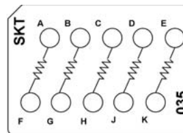
CTJ420E035 Five 10.2 kOhm Resistors, 1/10 W
