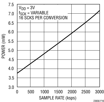
Figure 16. Power Consumption vs Sample Rate while the Device Remains Powered Up Continuously
