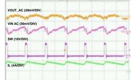
Switching State 3A Load
