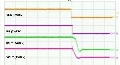
Power Good Falling 3A Load
