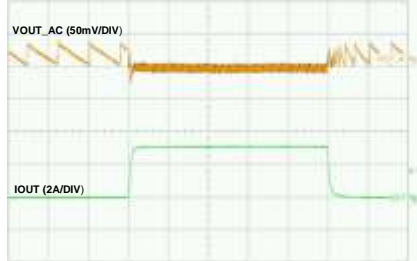
Load Transient Response (0 to 3A)
