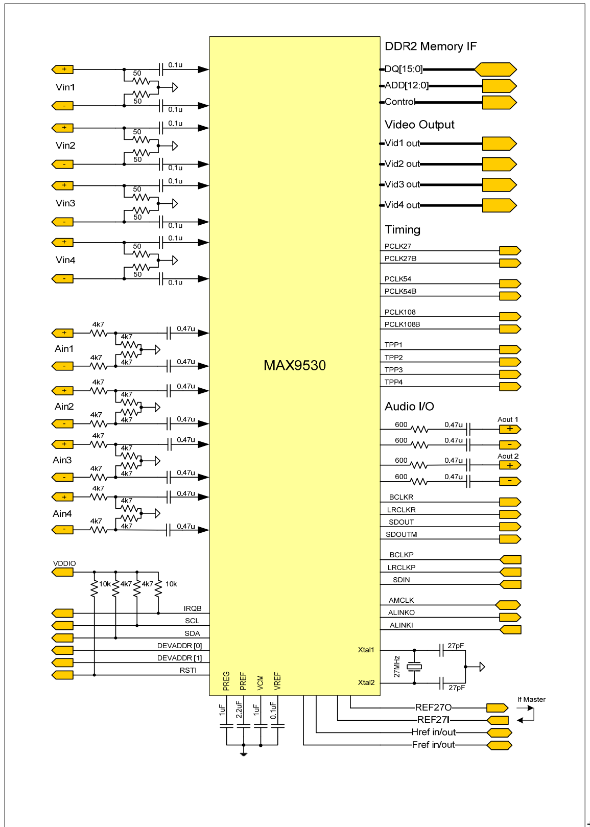
Figure 47: MAX9530 Typical application with differential inputs
