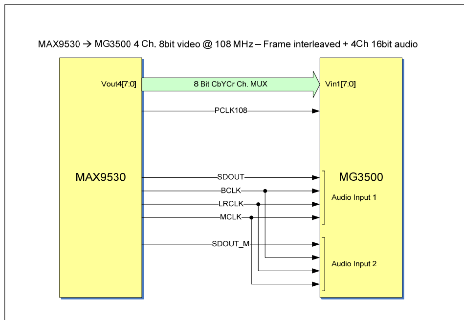
Figure 50: MAX9530 to MG3500 Interconnection [8bit Video @ 108MHz + 4 Ch.16bit audio]
