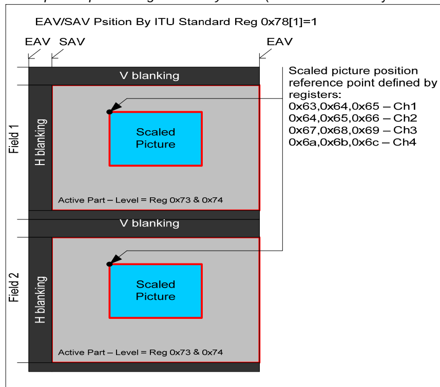
Figure 22: Scaled picture position in ITU mode – TRS (EAV.SAV are placed according to the ITU standard)
