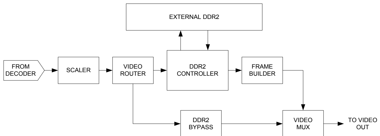
Figure 24: Frame Synchronization Module Block Diagram
