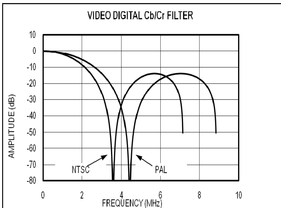
Figure 6: VIDEO DIGITAL Cb/Cr FILTER
