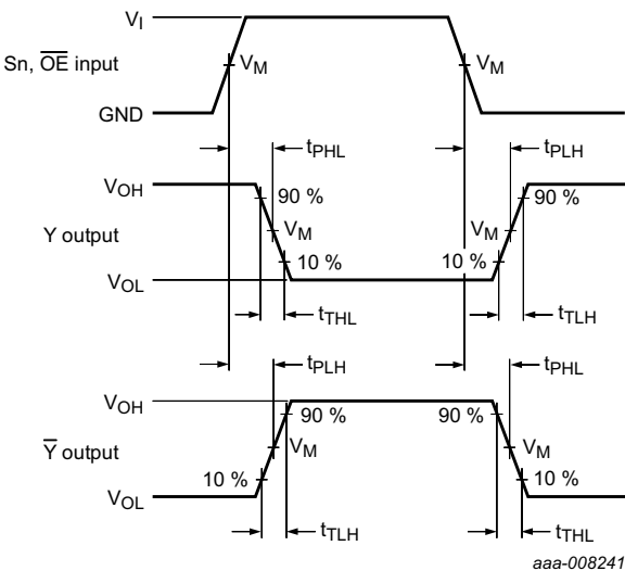
Measurement points are given in Table 8 . V_{OL} and V_{OH} are typical voltage output levels that occur with the output load. Fig 8. Propagation delay input (Sn, \overline{OE} ) to output (Y, \bar{Y} )
