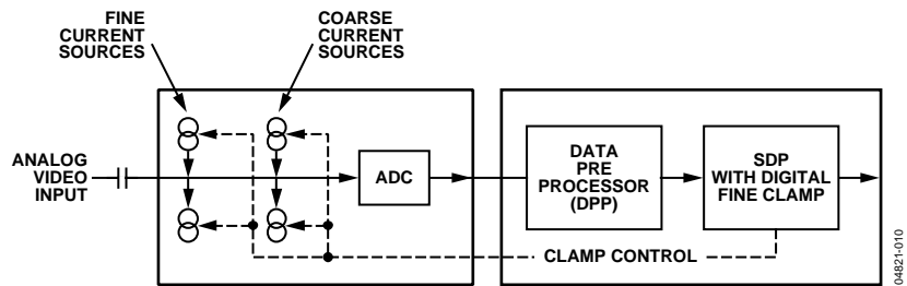
Figure 10. Clamping Overview
