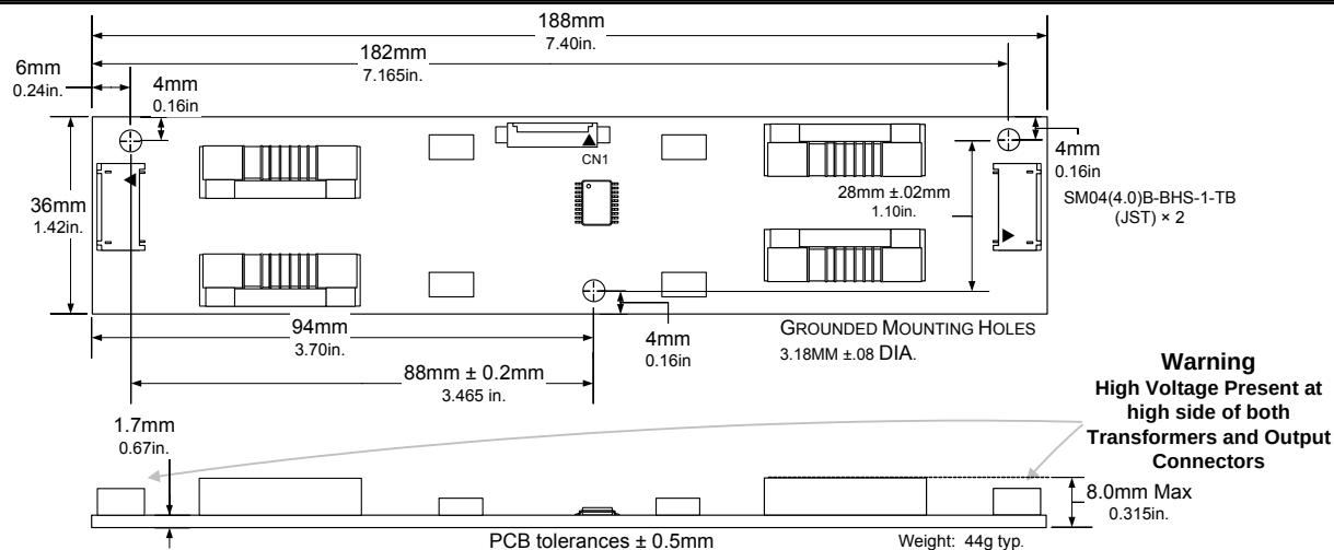
PHYSICAL DIMENSIONS
