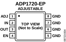
Figure 4. 8-Lead MSOP Pin Configuration—Adjustable Output Voltage
