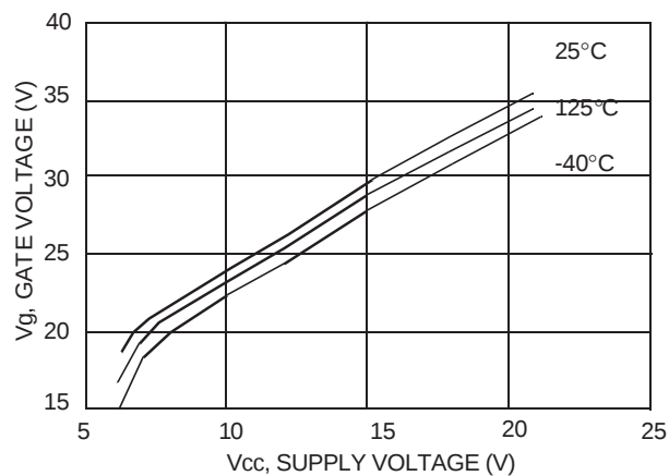
Figure 11. Gate Voltage versus Voltage
